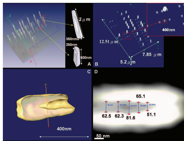
FIG. 2. (a) (Color) 3D rendering of tungsten plug with a keyhole and the diagrams showing the structure of the keyhole (right) and the tungsten plug with a 350 nm diam. (Right bottom) The tungsten plug with a 250 nm diameter. (b) The 3D rendering of the tungsten plug is plotted with higher threshold. The wire made of a copper-aluminum alloy is removed from the rendering; the tungsten distribution is shown. The red region of the left picture is the region of the right picture. The red region in the right picture is the tungsten plug, which is analyzed in (c). (c) The top view and side view of the tungsten plug displayed in a voxel mode (top) and an isosurface (bottom) mode. The orange line indicates the region of the cross-section plot that is shown in Fig. 3. (d) The measurement of the size of the keyhole. The diameters of the keyhole range from 50 to 80 nm.
